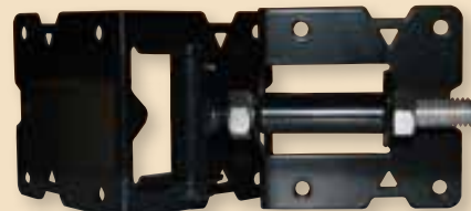
4 SS Black Hinge (Spring Loaded)
